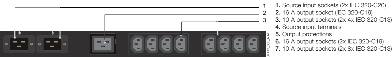
STATYS XS 16 A
